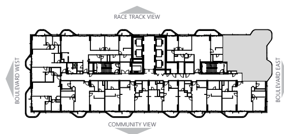
KEYPLAN - LEVEL 04 (TYP. ODD LEVELS UPTO L16)
