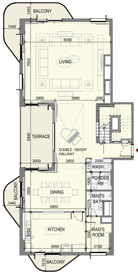
LEVEL 29
