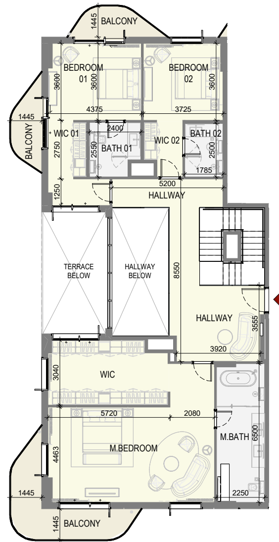
LEVEL 30
