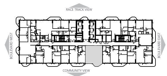
KEYPLAN - LEVEL 19 (TYP. ODD LEVELS UPTO L27)
