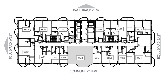
KEYPLAN - LEVEL 03 ( TYP. ODD LEVELS UPTO L17)
