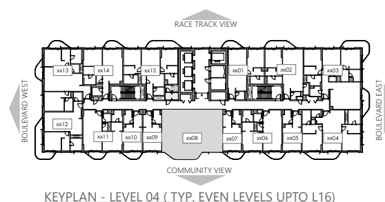
KEYPLAN - LEVEL 04 ( TYP. EVEN LEVELS UPTO L16)
