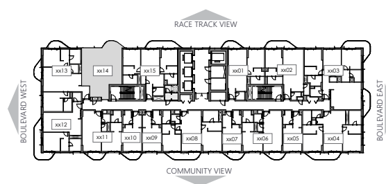
KEYPLAN - LEVEL 04 ( TYP. EVEN LEVELS UPTO L16)
