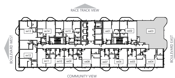
KEYPLAN - LEVEL 04 ( TYP. EVEN LEVELS UPTO L16)
